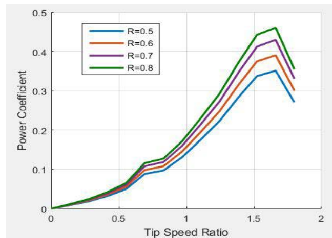
Figure 4. Effect rotor radius on power coefficient.
