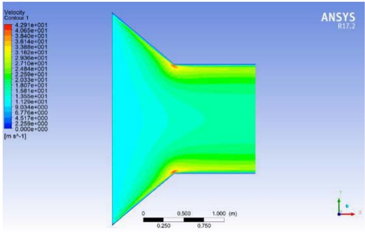
Figure 11. Flow velocity in the convergent model of inlet angle 40°.
