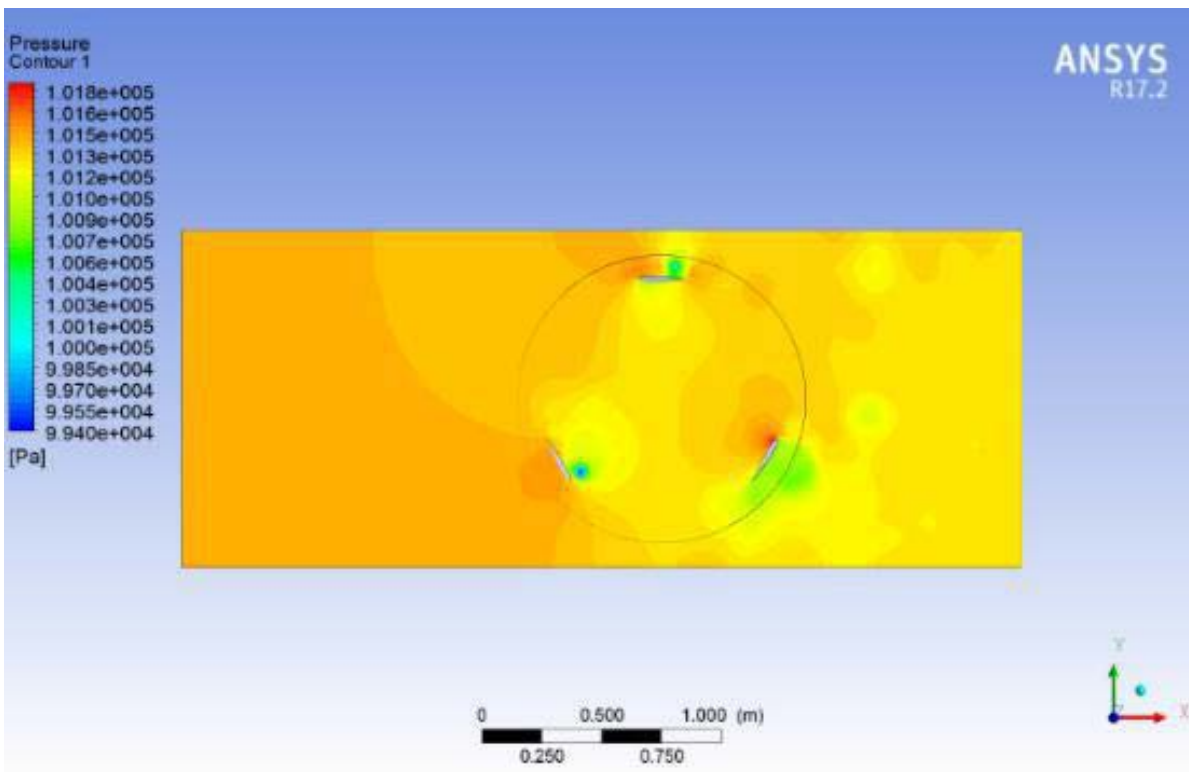
Figure 13. Variation of pressure in non-ducted vertical axis wind turbine.
