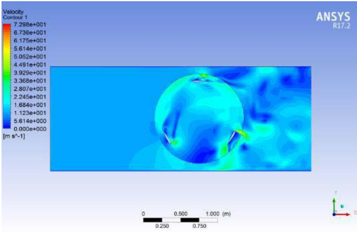
Figure 12. Velocity distribution in the non-ducted vertical axis wind turbine.
