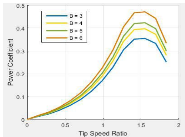
Figure 5. Blade number (B) influence on the power coefficient.
