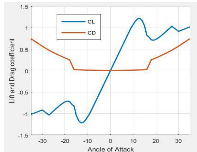
Figure 3. Drag and lift coefficient changing with angle attack.
