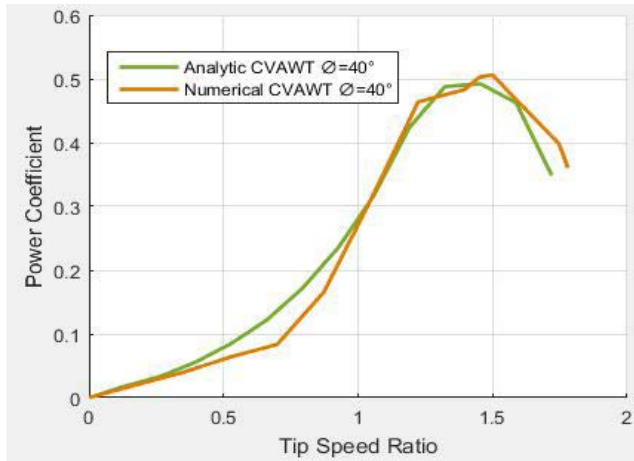
Figure 16. Power coefficient with TSR.
