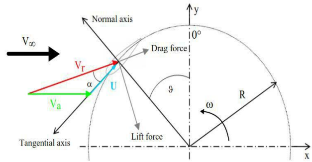
Figure 1. Velocities and flow blade angles 11 .
