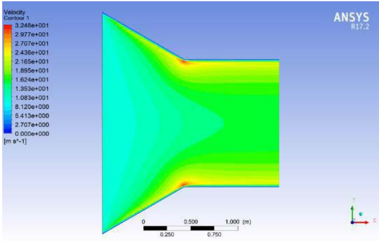
Figure 10. Flow velocity in the convergent model of inlet angle 30°.
