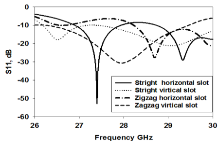
Figure 4. The reflection coefficient of SIW antenna
