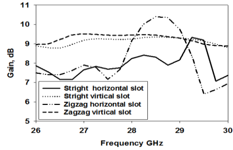
Figure 5. Gain of SIW antenna
