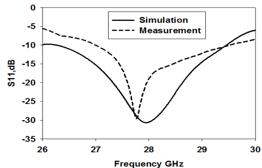
Figure 8. Comparison the reflection coefficient between simulation and measurement of SIW antenna which has zigzag slot
