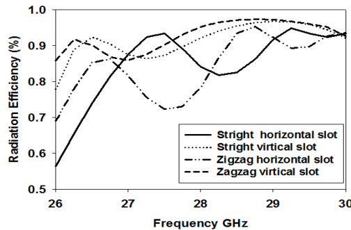
Figure 6. The radiation efficiency of SIW antenna
