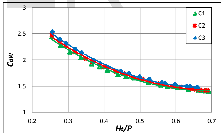
Figure 6 Variation of free overflow discharge coefficient ( C_{dw} ) versus H/P for various \Delta P/P of PKW type C.
