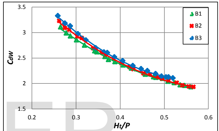
Figure 5 Variation of free overflow discharge coefficient ( C_{dw} ) versus H/P for various \Delta P/P of PKW type B.
