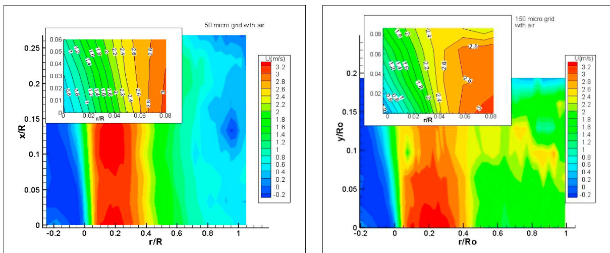
Figure 4. Axial velocity downstream the nozzle with 50 µm (left) and 150 µm (right).
