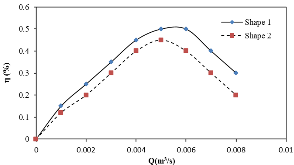
Figure 6. Pump efficiency variation with flow rates for different impeller blades
