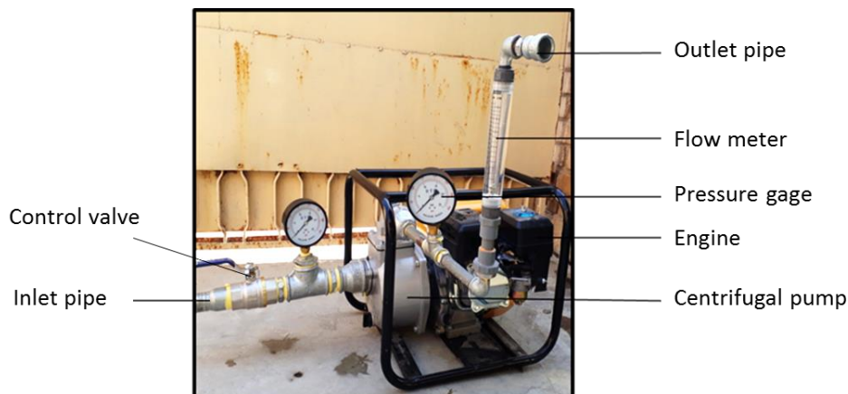
Figure 2. Test rig layout
