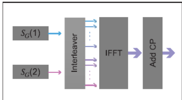
Figure 8. General S-SCH Symbols [5].
