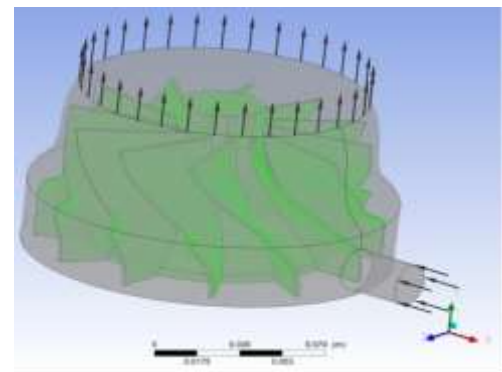
Figure 8: Boundary condition
