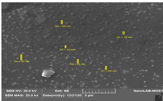
Fig.2: Micrograph of the electron microscope (SEM) demonstrates the size and shape of synthesised silver nanoparticles (AgNPs).
