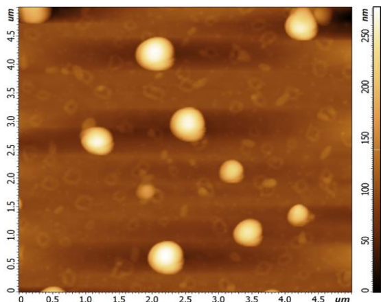
Fig.3: The atomic force microscopy's (AFM) result demonstrates the two dimensions of silver nanoparticles (NPs).
