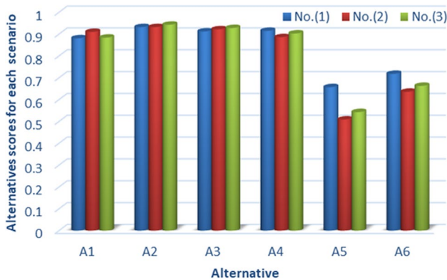
Fig. 4 Alternatives Scores for each Scenario resulting from the WPM method
