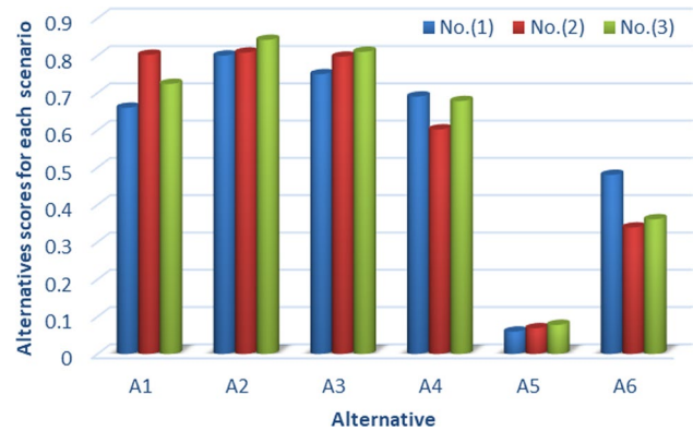
Fig. 5 Alternatives Scores for each Scenario resulting from TOPSIS method
