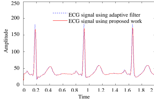
Fig. 7: ECG signal for three times based on classical and proposal approach
