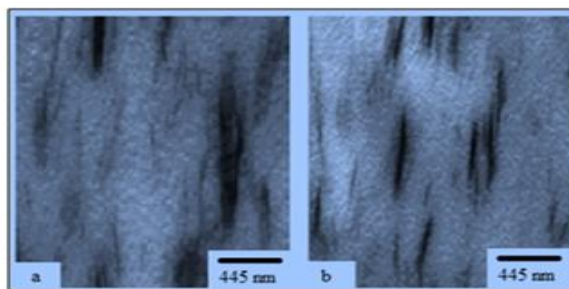
Fig. 4: TEM of a) PBS/PCL blend and b) PBS/PCL-OMMT nanocomposite
