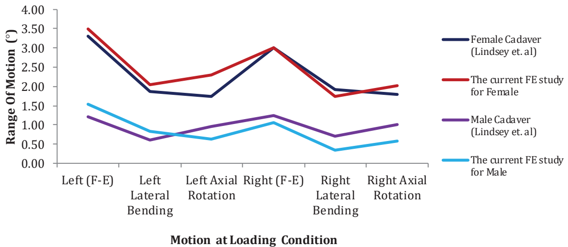
Figure 1. Validation results for the intact female and male lumbar segment-sacrum (right and left sides) at 7.5 N.m moment under loading condition. Experimental data was taken from Lindsey et al. [14].
