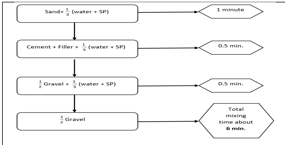
Fig. 1. Mixing Procedure.
