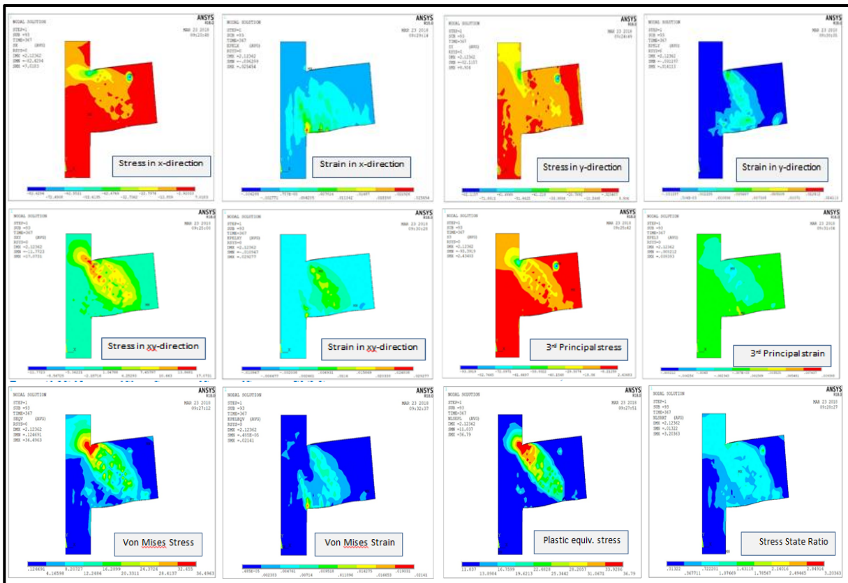
Fig. 13. Numerical Stresses and Strains for Specimen C3(0.9).
